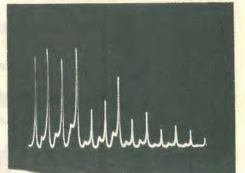
Fig. 3. Same comb as in Fig. 2, but after correction for linearity. Note improvement in spacing between the spikes on the right-hand side. Display covers 100 to 200MHz with 10MHz spacing.
