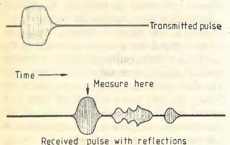
Fig. 5. In suppressing echoes by pulse technique, the transmitted pulse is short enough to allow the received signal to be measured before the arrival of reflections.
