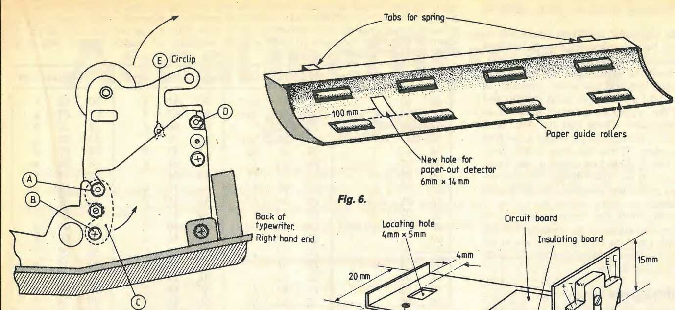
Fig. 5. Platen roller must be swung upwards to allow access for fitting the paper-out detector. Remove screw B on the right-hand roller support bracket. Swing plate C clear on the right-hand bracket and swing the platen roller assembly upwards, pivoting it about nut D.
