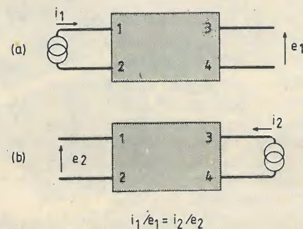
Fig. 1. Four-port network is reciprocal if its transfer admittance is the same in both directions.
