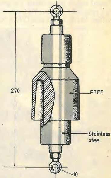
Fig. 10. Tough German aerial strain insulator using skirt principle. Rated at 50kV (dry) at 500kHz. 700kg tensile load, mass 1.5 kg. (Dieckmann & Klapper.)
