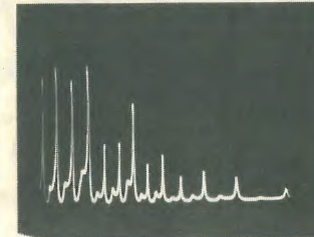
Fig. 2. Output from a typical comb generator as seen on the home-made spectrum analyser. Uneven spacing between the 'prongs' is corrected by adjustments described in the text; height difference is unimportant. Bumps at the bases of the spikes may indicate tuner overloading.
