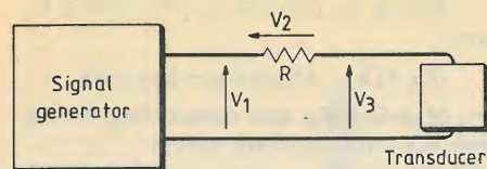
Fig. 3. In the absence of a bridge the input impedance of a transducer may be determined by measuring the voltage drop across a series resistor.
