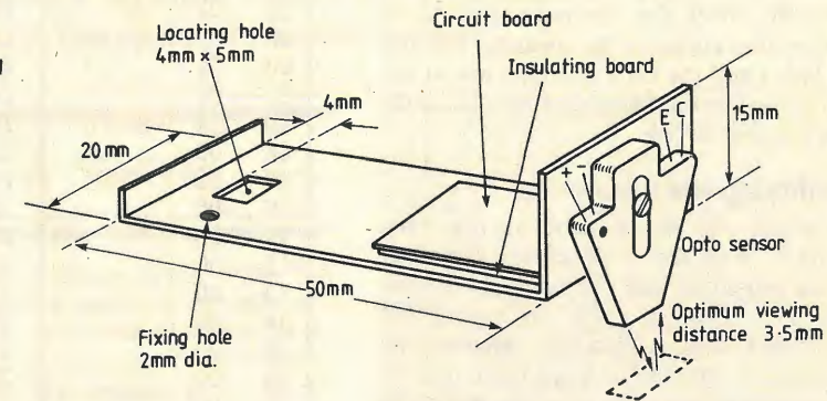
Fig. 7. Opto-sensor mounted underneath the platen roller views the paper through a hole cut in the paper guide roller carrier (Fig. 6).
