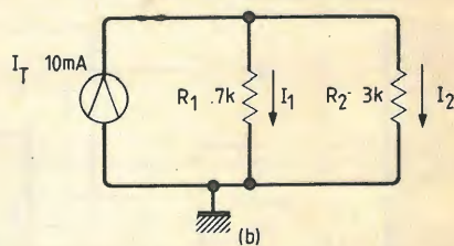
Fig. 2. Current dividers formed with parallel branch resistors.
