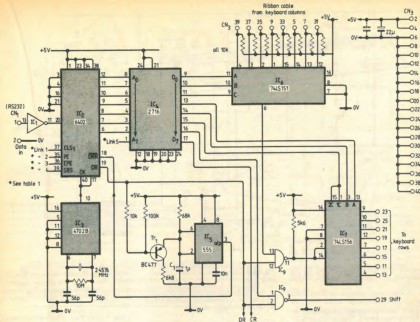
Fig. 2. Incoming serial data from the computer is converted by the interface into parallel data in a form suitable for connection to the keyboard matrix of the typewriter. IC 1 is a section of an MC1489 line-receiver device.
