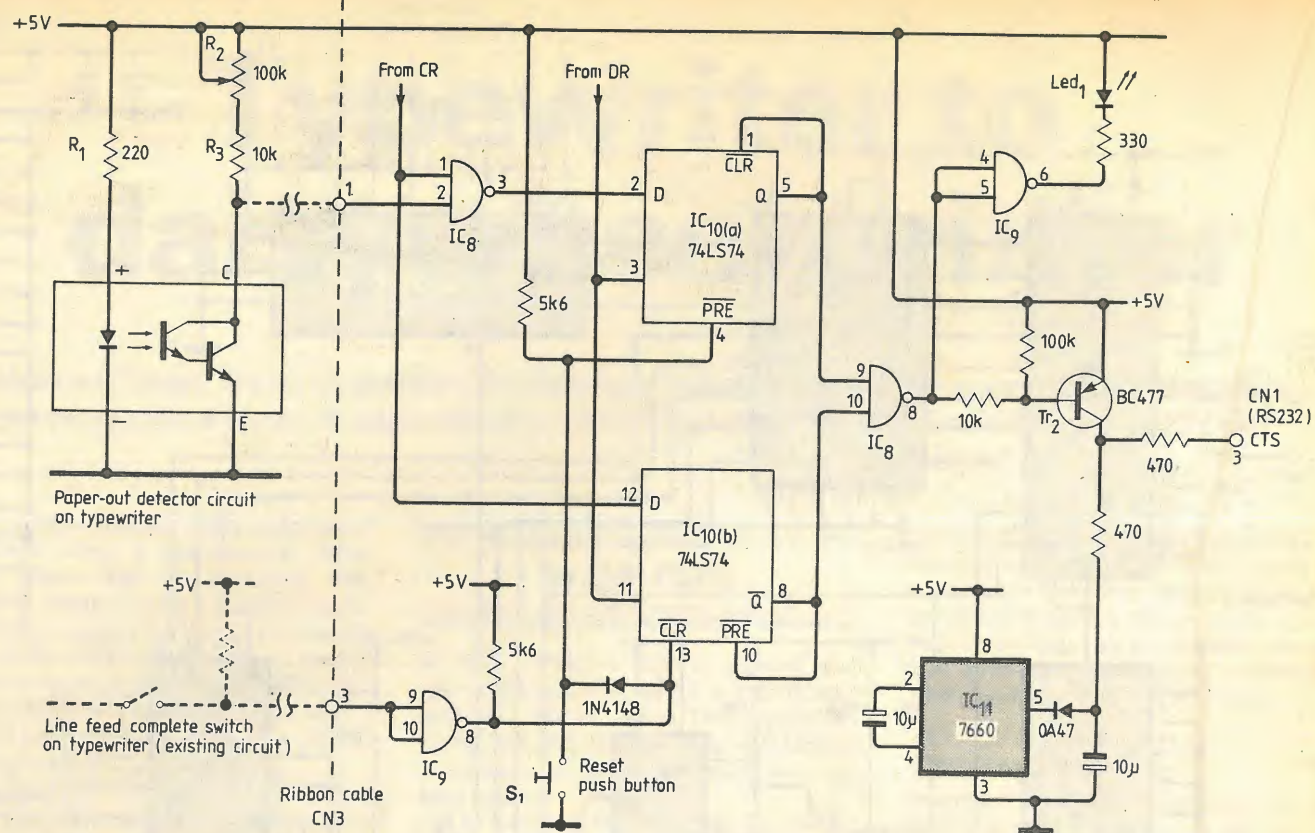
Fig. 3. Output from the computer is halted by this sensor circuit when the paper runs out. This feature is often not provided even on high-cost printers. IC 8 is a 74LS132 and IC 9 a 74LS03. A suitable opto-switch is type 307-913 from RS Components.
