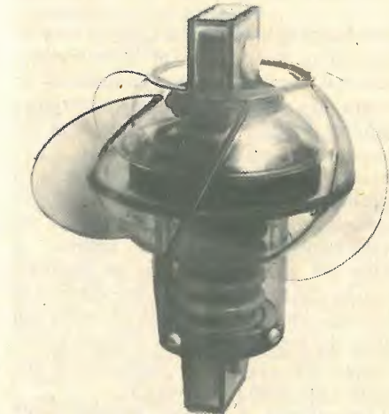
Fig. 14. British invented link/strain insulator assembly with protective shrouding. Wind-driven rotating outer dome expels water by centrifugal action. (P. F. Barber, Scarborough.)
