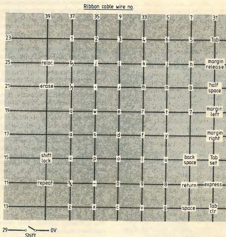
Fig. 1. Typewriter keyboard matrix: columns are each pulsed low in turn and pressing a key connects a column to a row. For clarity, diagram shows lower-case characters only.
