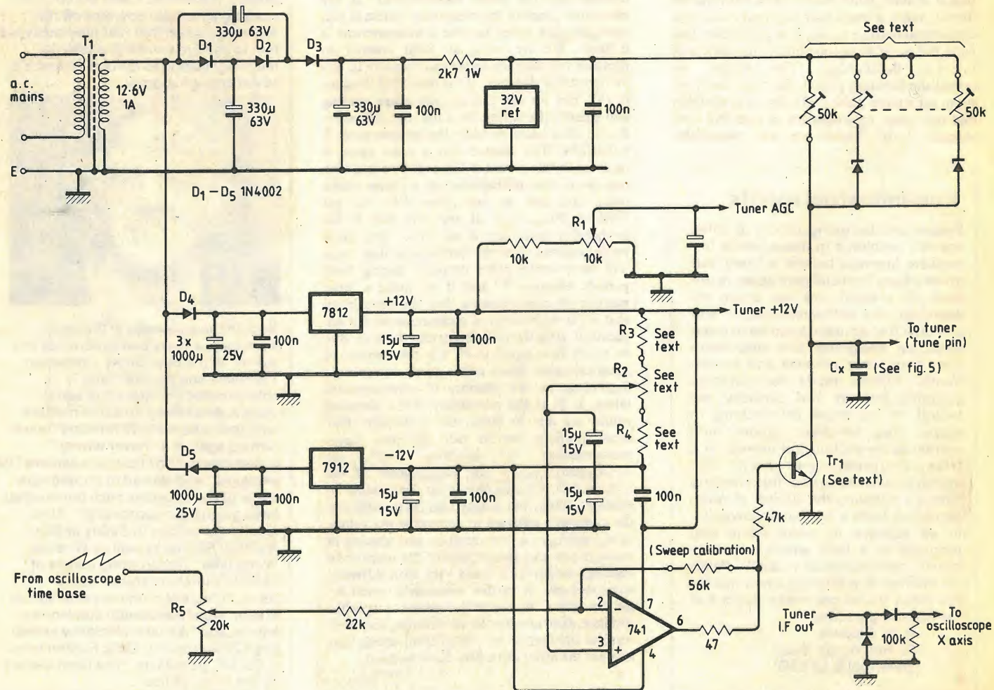
Fig. 1. Power and control-voltage supplies for the tuner module. Tuner is swept across its range by a waveform derived from the timebase of an oscilloscope; after rectification its i.f. output is applied to the vertical deflection input. Network at the collector of Tr 1 provides correction for the non-linearity of the tuner's tuning characteristic.
