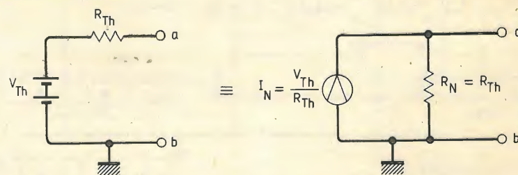
Fig. 4. Finding the Norton circuit from the Thévenin circuit.
