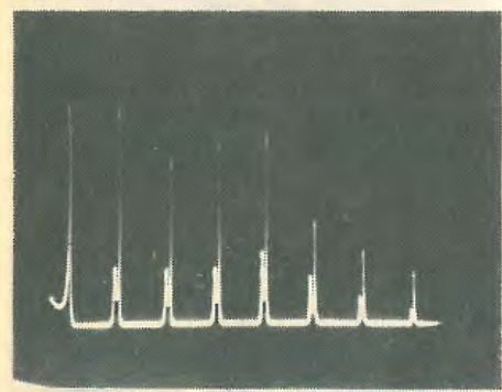
The same linearity correction should be effective on more than one band. This shows a u.h.f. display from 500 to 850MHz with 50MHz spacing.
