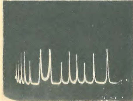
If the oscilloscope sweep speed is too fast, as it is here, the tuner frequency may still be dropping when the next sweep begins. This can arise because voltage-controlled tuning circuits usually incorporate some capacitance for stability, for example, C x in Fig. 1.
