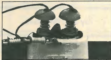
Fig. 6. Traditional British feedthrough set-up, unchanged since the days of silent movies, photographed in 1983.
