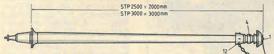
Fig. 8. German 10-foot-tall glass-fibre feedthrough trunk shown on its side. Intelligent design, efficient and unobtrusive. Requires no safety fencing. Might benefit from a few rain cones along the shaft. Dieckmann & Klapper, Gerätebau GmbH, Hamburg.)
