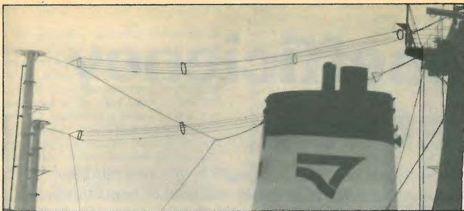
Fig. 4. Hard-to-find classic French all-wire sausage aerials with high top capacitance, well sited on available structures. ('Dumont d'Orville,' French flag, b.1977, 23910 g.r.t. photographed at Cr. Couronne, 1983.)
