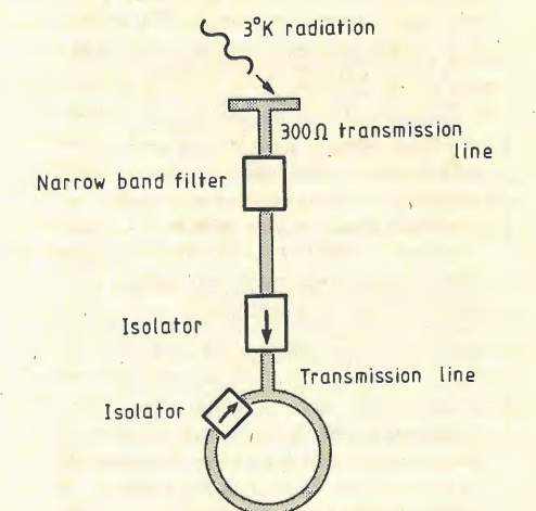
Fig. 2. More practical arrangement for putting the wave into the circular line.
