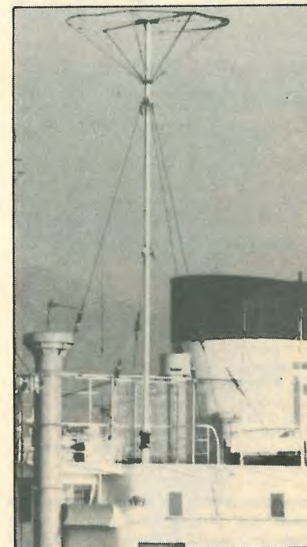
Fig. 3. Top-loaded unipole aerial of Scandinavian origin. The stays add to the top capacitance, also to the leakage. Has little height. (Photographed at Eleusis, Greece, 1982)
