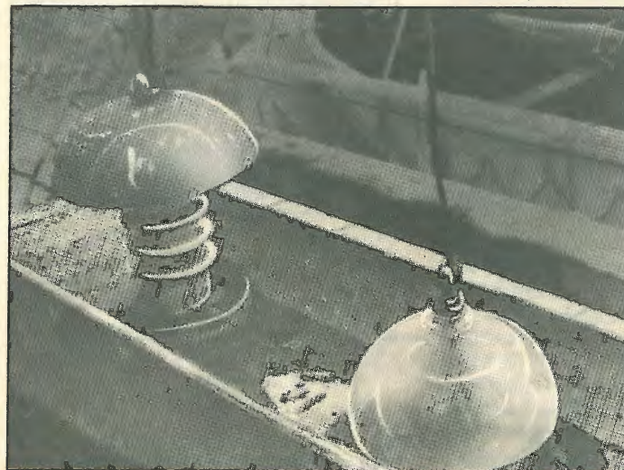
Fig. 15. Sea trials with one feedthrough protected, the other traditional. In later trials protected link insulators added.
