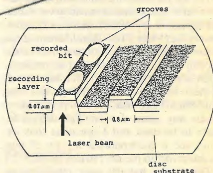
An erasable optical storage disc for video images and data developed by Matsushita uses two separate lasers for recording and erasing through a common optical system. The one gigabyte disc can record broadcast pictures in real time and be erased over one million times but when the disc might be available is not yet certain.
