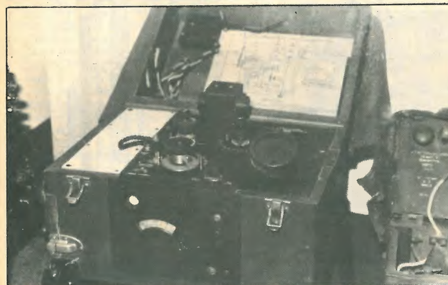
Fig. 1. This l.f. trench transmitter operated into an aerial only a metre above ground, but others worked from aerals inside the trench. (20watt Mk 3 transmitter, 1917, has single-valve tuned-anode oscillator, but a second valve could be switched in parallel for maximum power. HT supplied by 1,000-volt battery or induction coil.)
