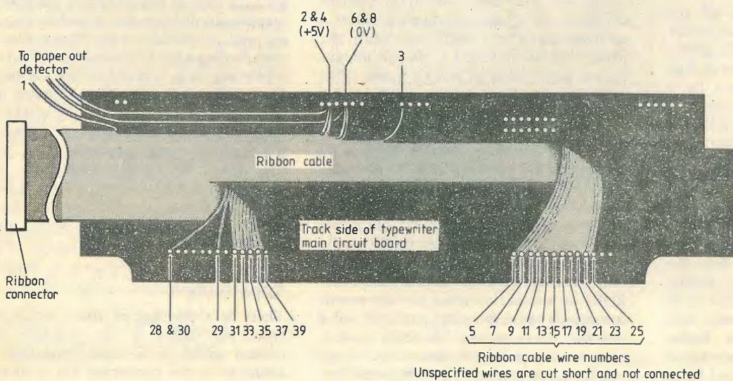
Fig. 4. 40-way ribbon cable connects the interface to the underside of the typewriter main circuit board. Alternate wires in the ribbon are connected to +5V or 0V either at the interface end or the typewriter end. This helps to prevent crosstalk between the signal wires.
