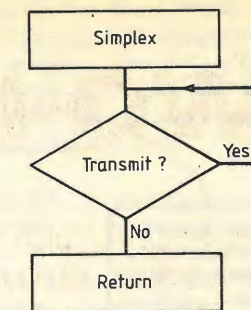
Simplex subroutine
