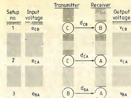
Fig. 2. Schematic three transducer reciprocity calibration. Drive voltage e_{CB} is applied to transducer C, which transmits to transducer B, at a distance d_{CB} , giving an output voltage v_{CB} . Test is repeated with C transmitting to A and B transmitting to A.
