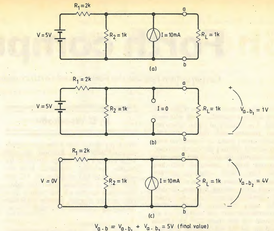
Fig. 6. Using superposition with a current and voltage source. Original circuit (a), circuit with current source open (b), and circuit with voltage source shorted (c).
