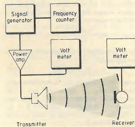
Fig. 4. Minimum instrumentation is a signal generator and suitable power amplifier, a frequency counter and a means of monitoring the transmitter drive level and receiver output voltage.
