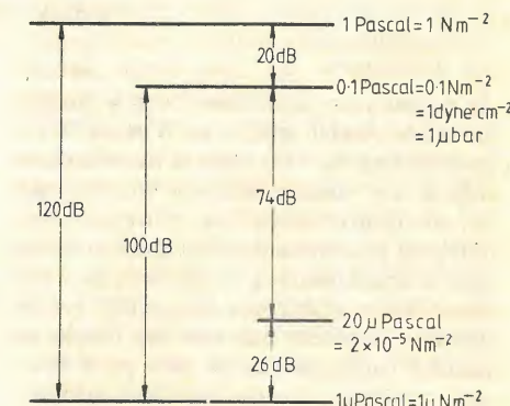
Reference pressure levels in common use and the relationships between them.
